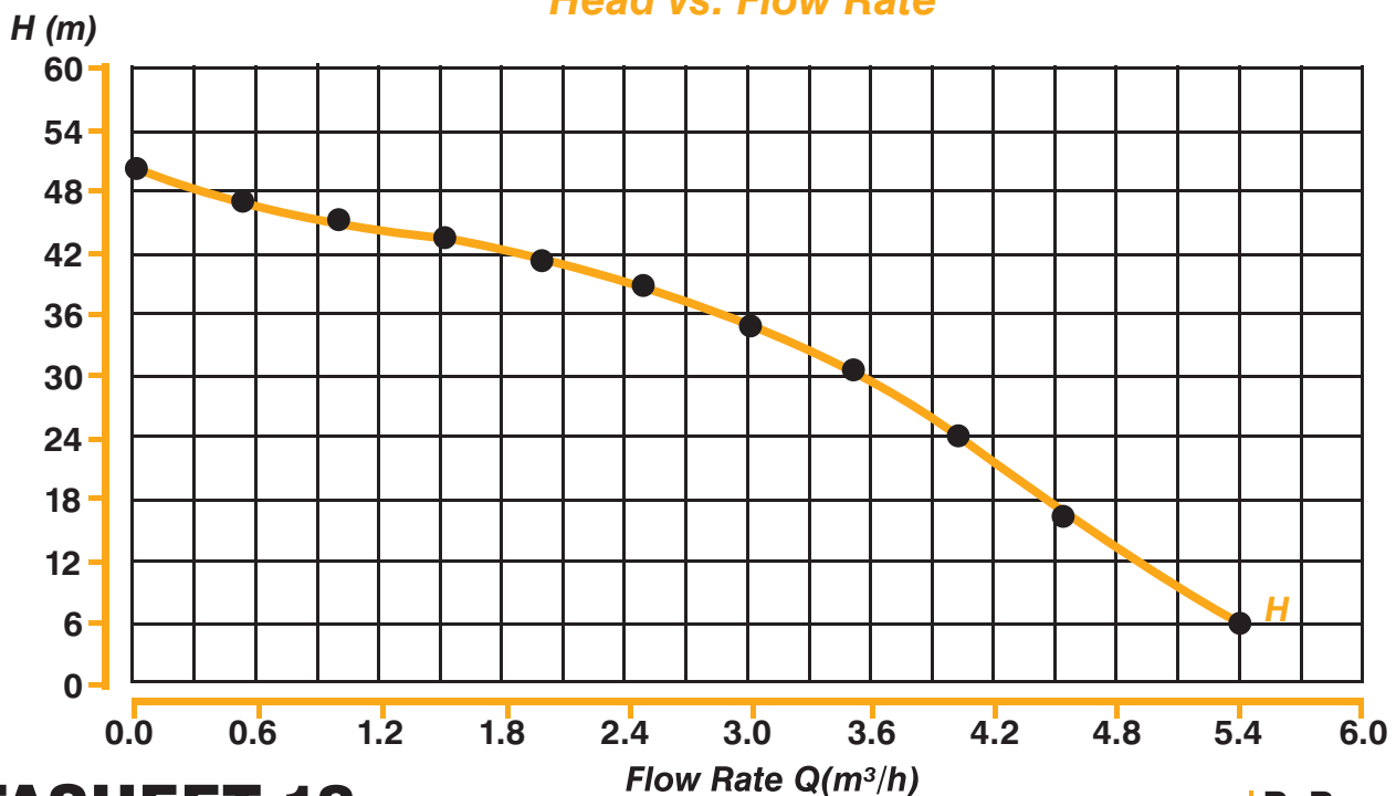
Head vs. Flow Rate
